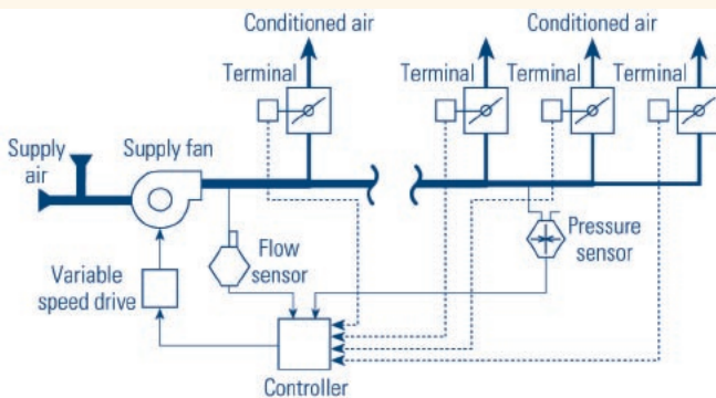
Figure 1: Schematic of a variable-air-volume air handling system. Conventional variable-air-volume systems cut energy use by reducing fan power at part-load conditions, but save less than they could because they maintain a constant supply duct static pressure.
